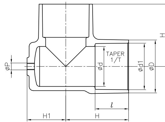
65–150 mm Injection Molding
