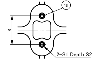
View A
